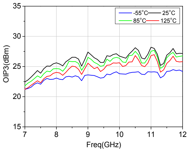
OIP3 vs Frequency
