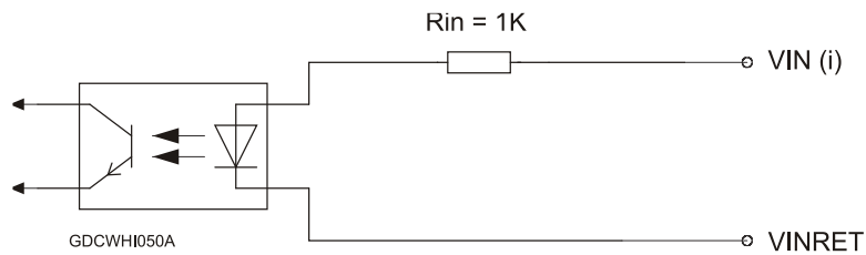
Figure 39: Digital Input TTL Schematic
