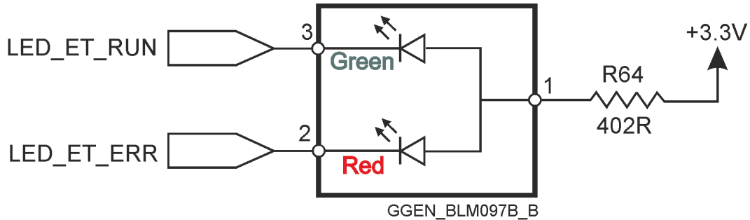
Figure 59: EtherCAT Status Indicator
