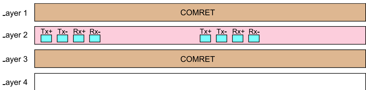
Figure 60: Example of Layered Stackup on PCB
