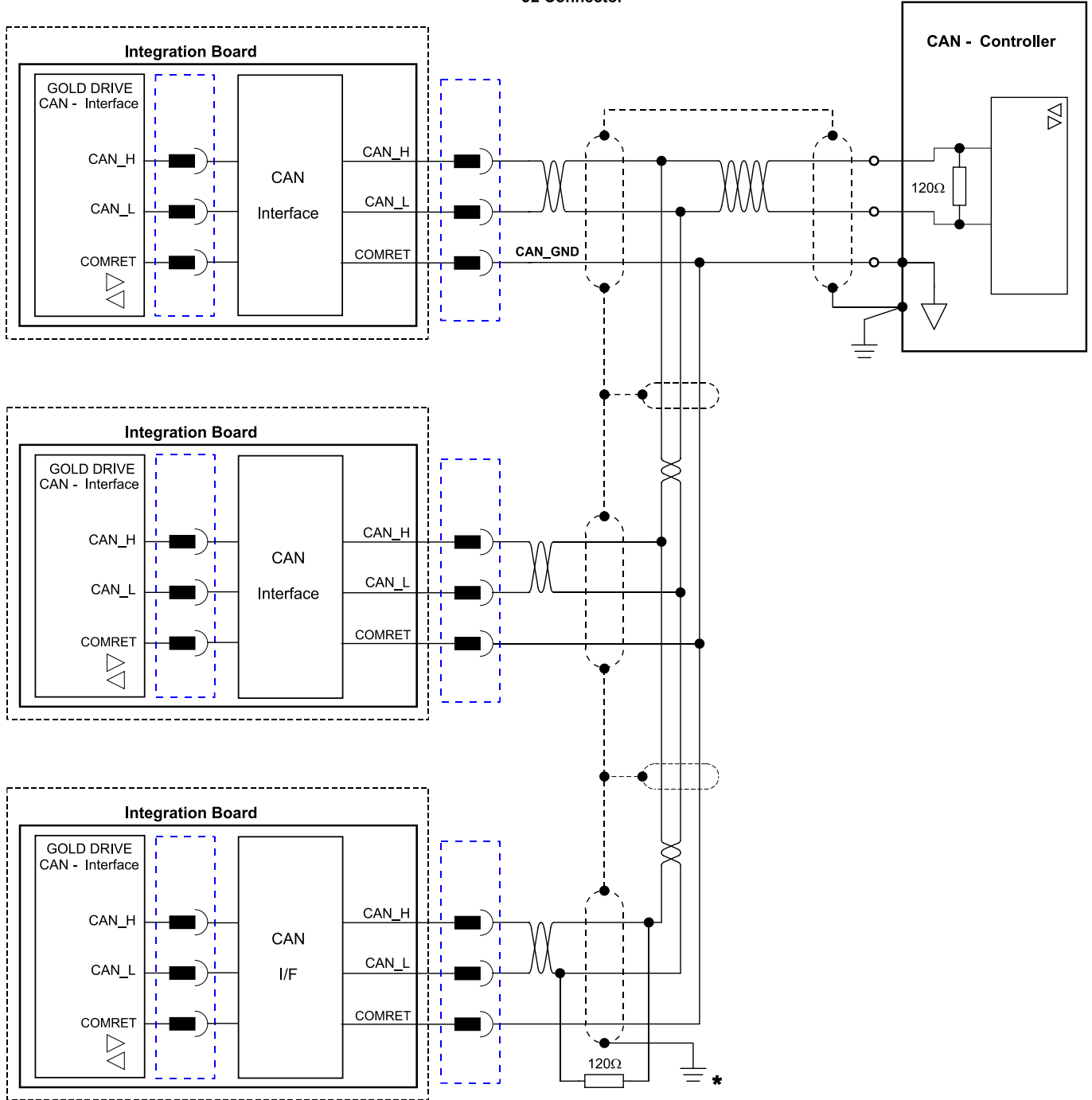
Figure 62: CANbus Connections
