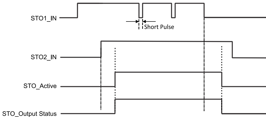
Figure 20: STO Output Status Timing Diagram
