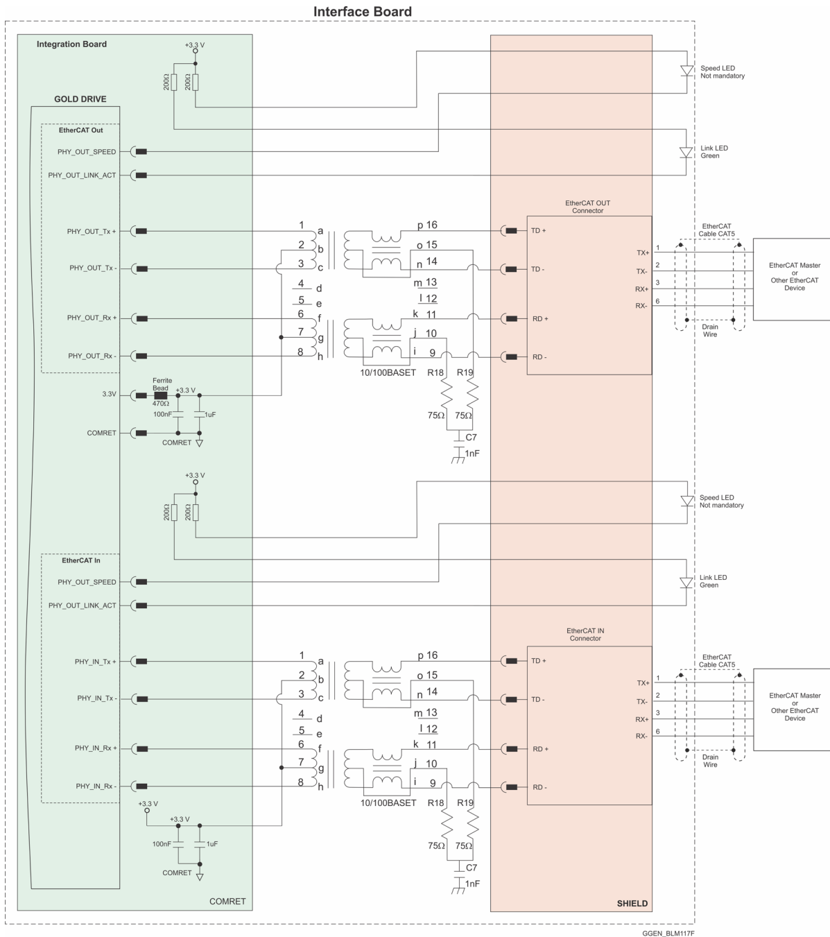
Figure 58: EtherCAT Connection Schematic without Magnetic Diagram
