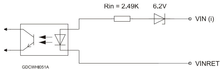
Figure 45: Digital Input Source Schematic
