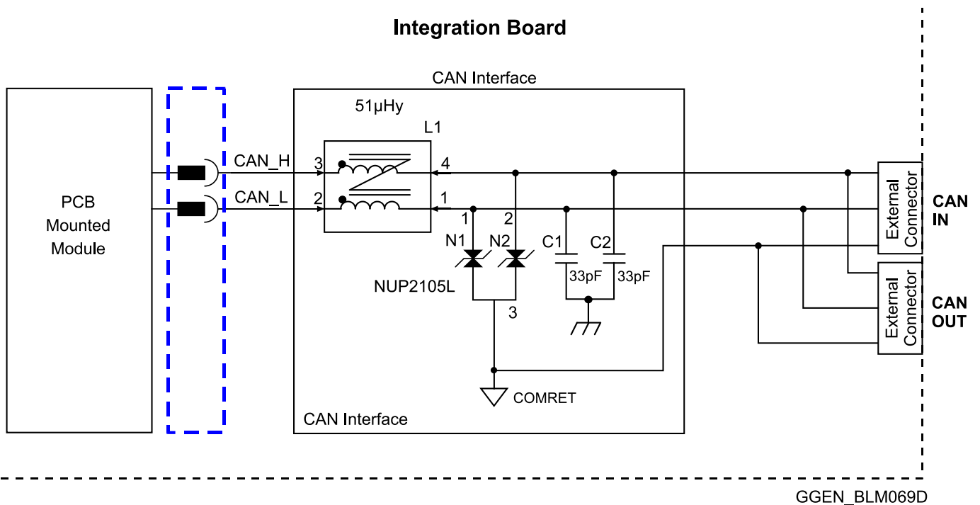
Figure 63: CAN Interface
