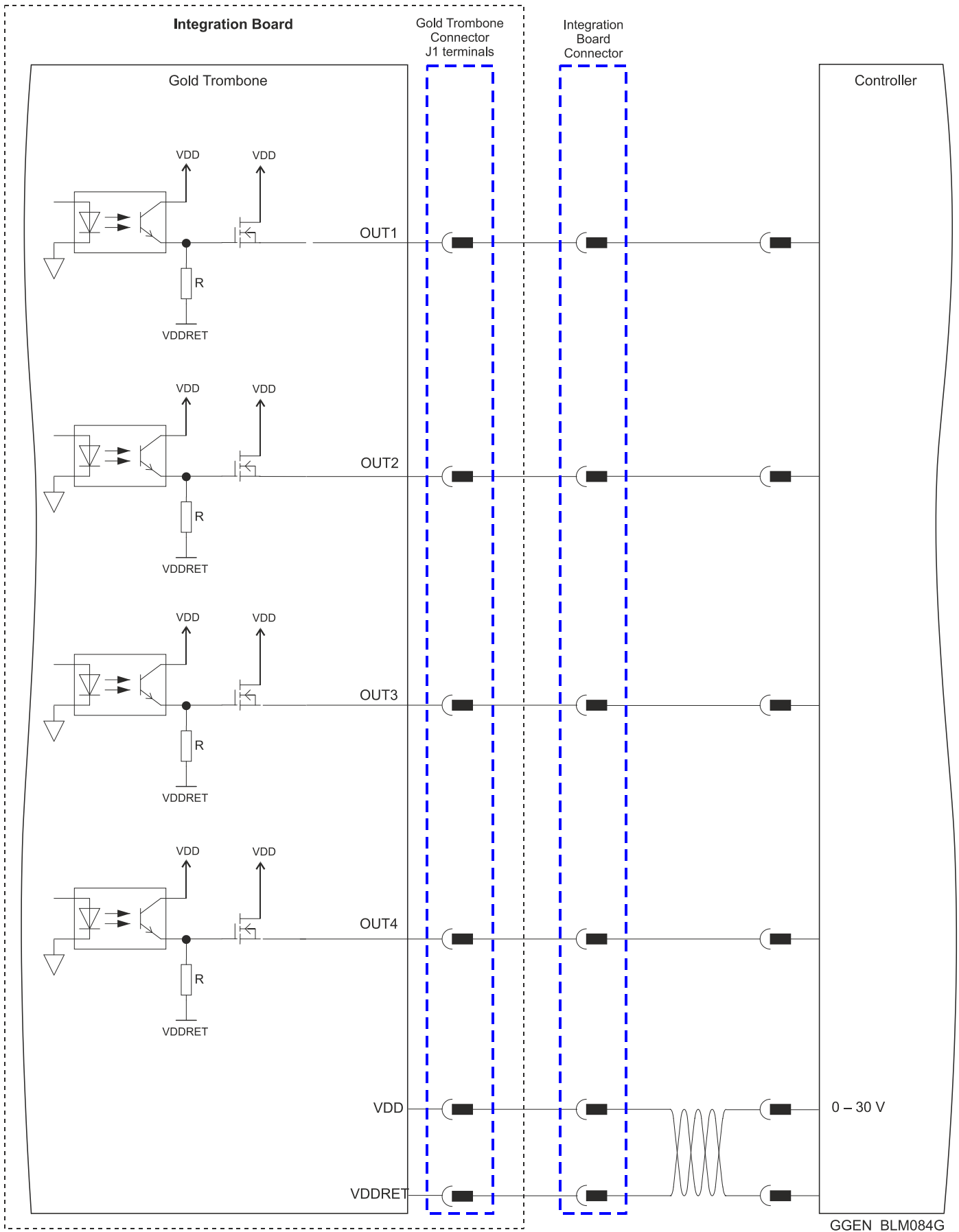
Figure 50: Digital Output Connection Diagram
