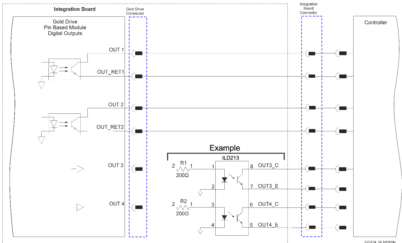
Figure 42: Digital Output Connection Diagram – TTL Connection
