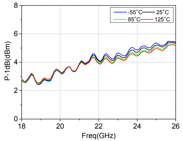
Output P-1dB vs Frequency
