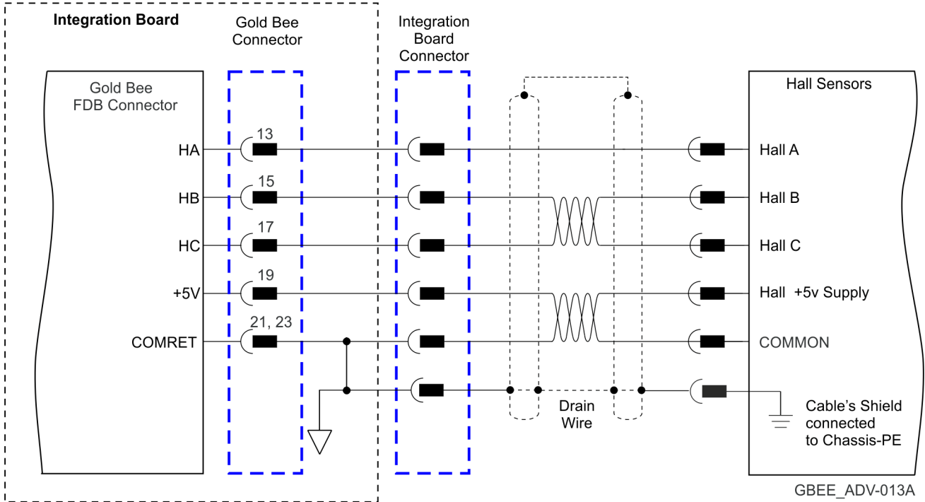
Figure 14: Hall Sensors Connection Diagram
