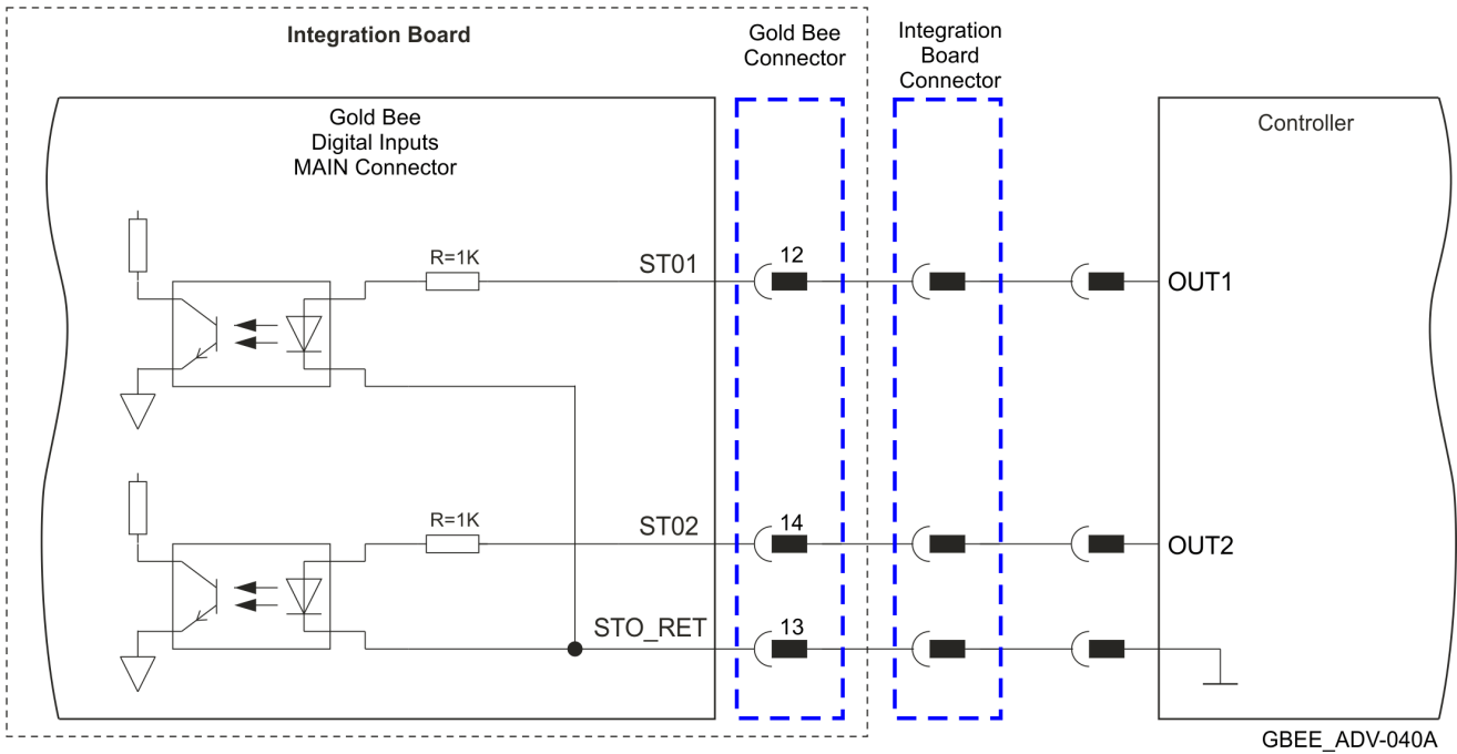
Figure 22: STO Input Connection – 5V Logic Level
