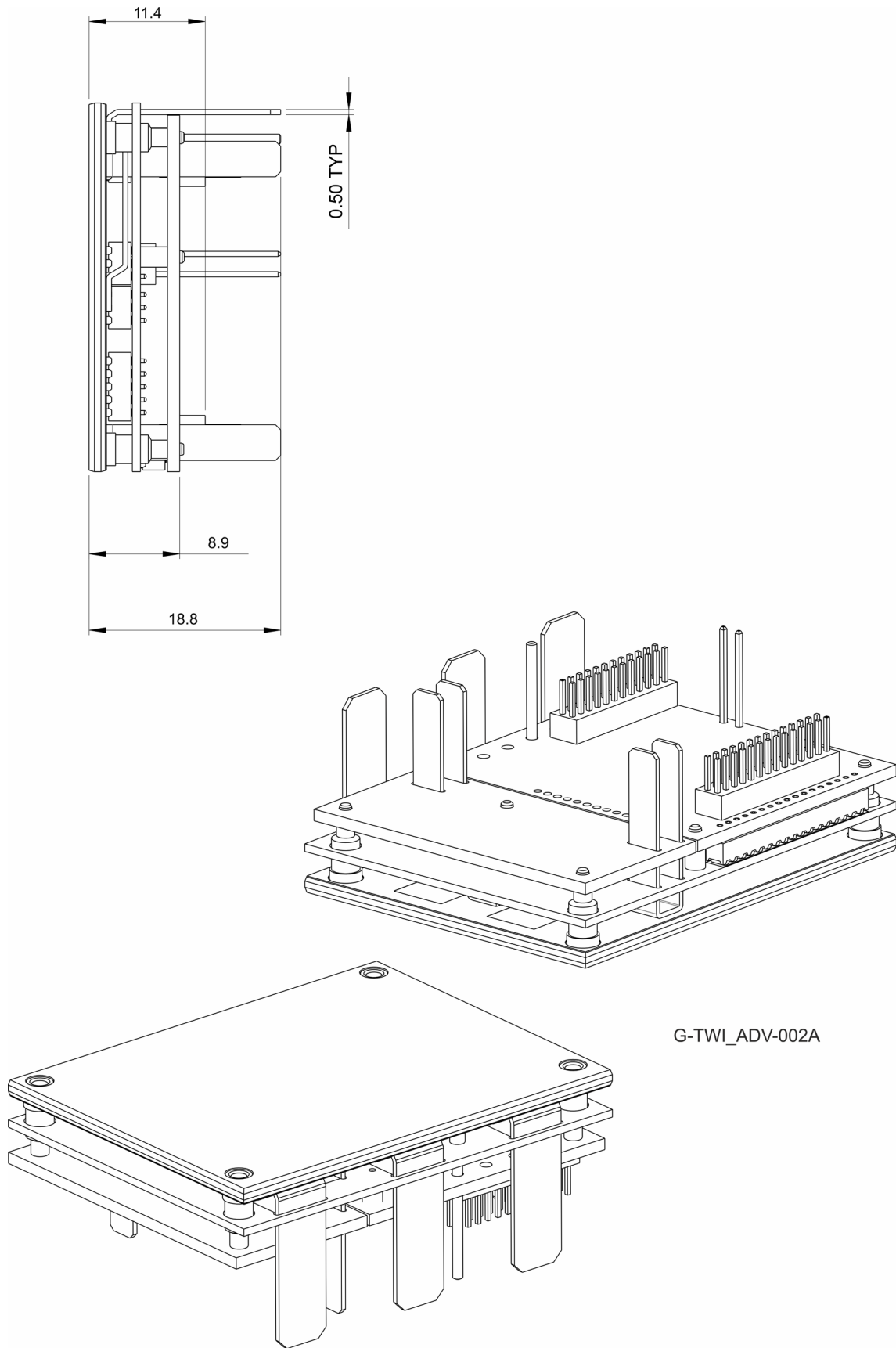
Figure 32: Gold Bee EtherCAT version
