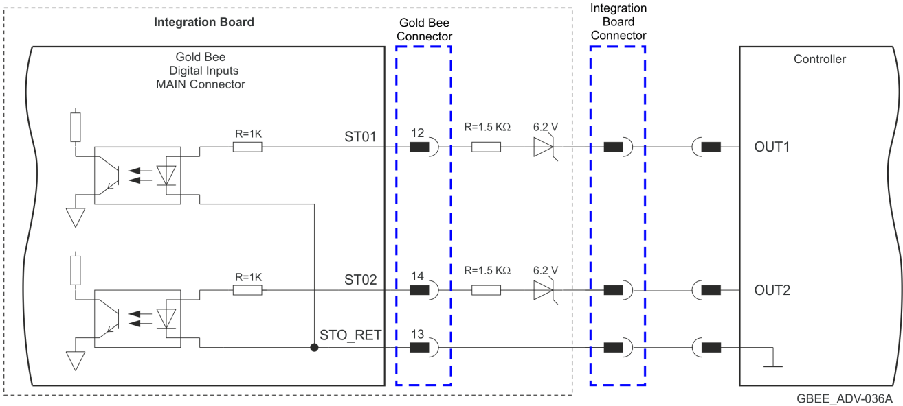
Figure 23: STO Input Connection – PLC (24V Logic)
