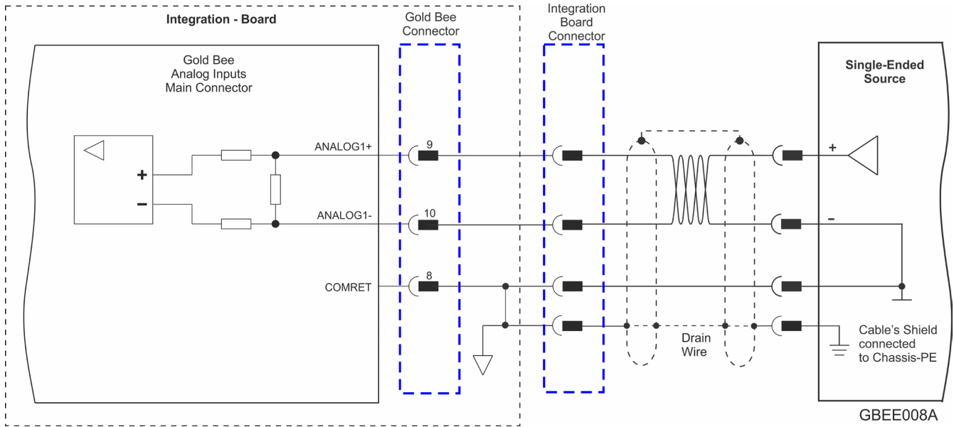
Figure 24: Analog Input
