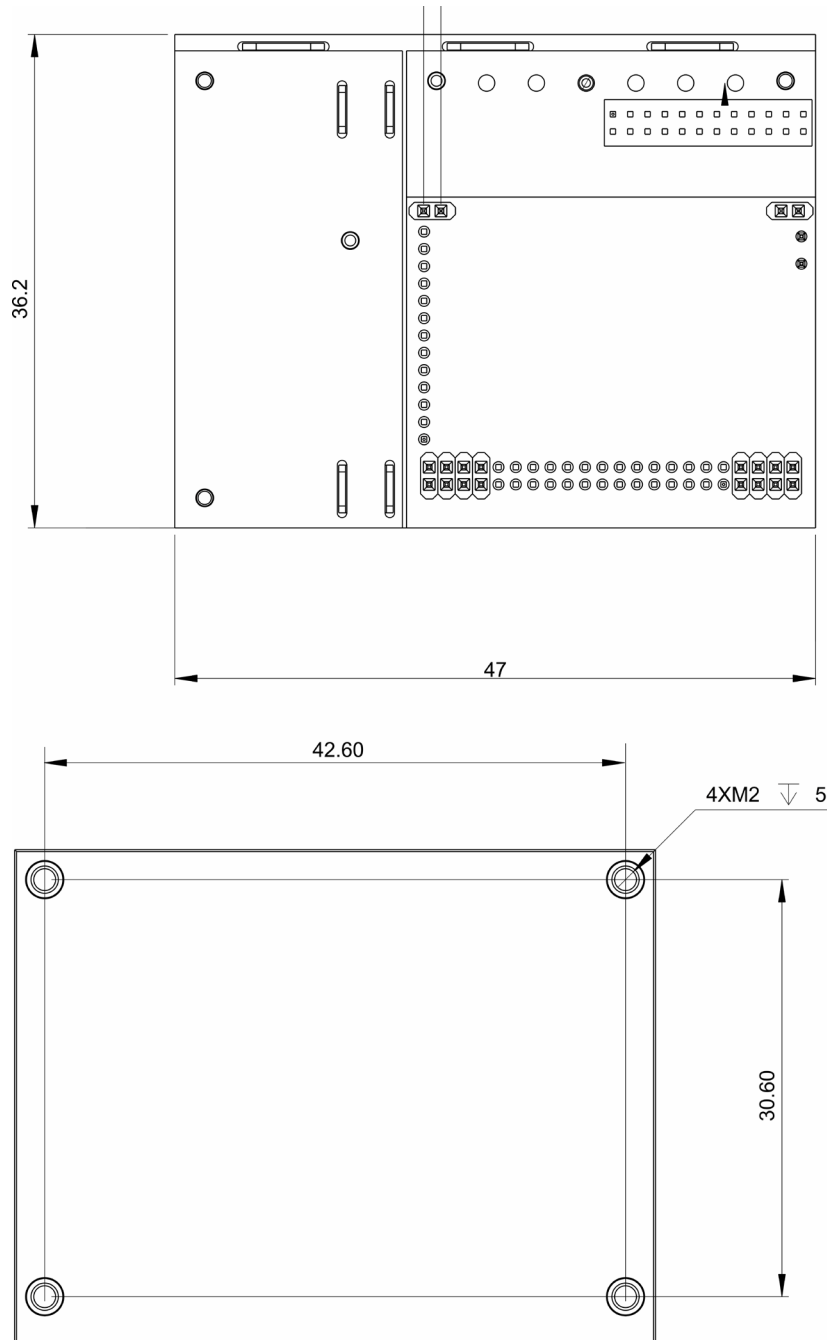
Figure 2: Gold Bee Version Dimensions
