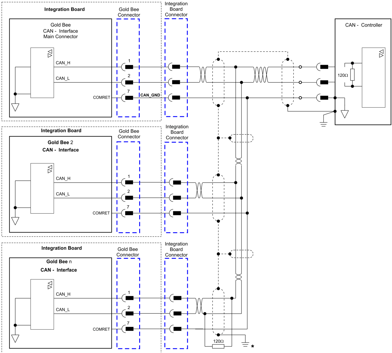
Figure 26: CAN Network Diagram
