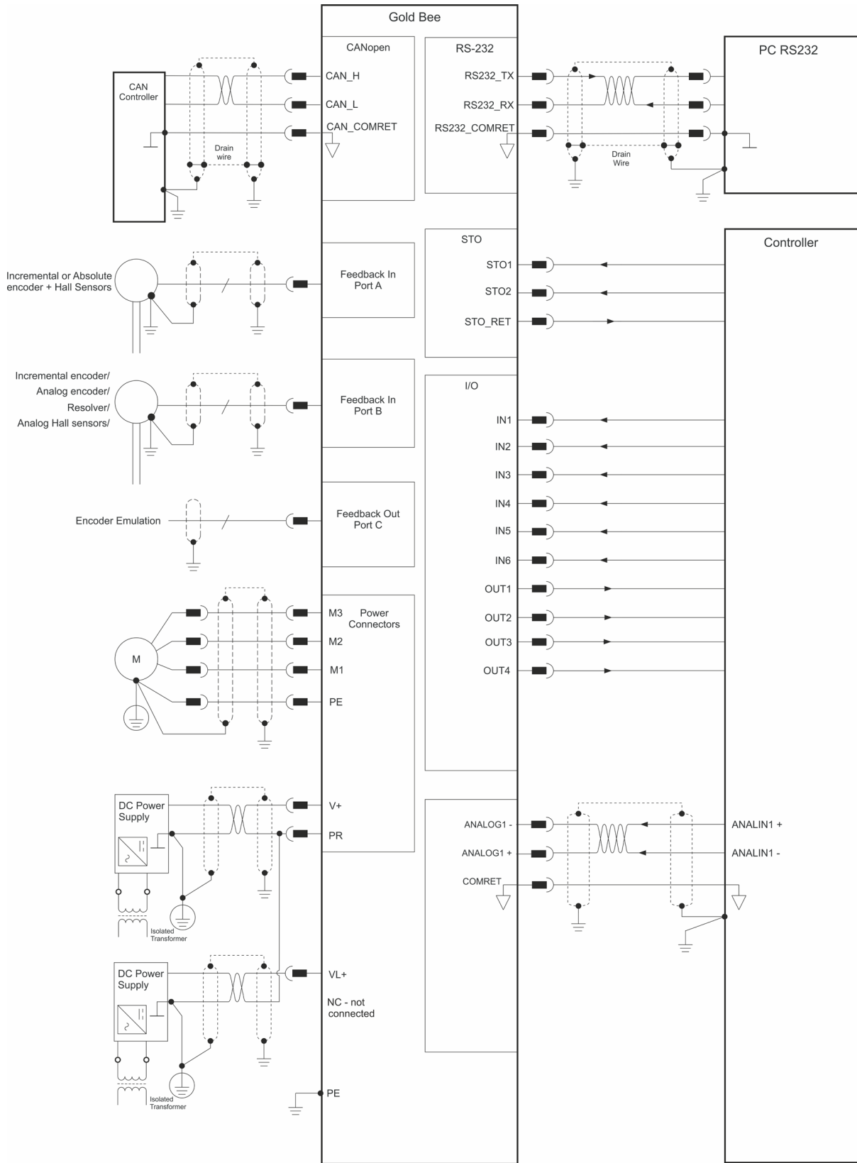
Figure 3: The Gold Bee CAN Connection Diagram
