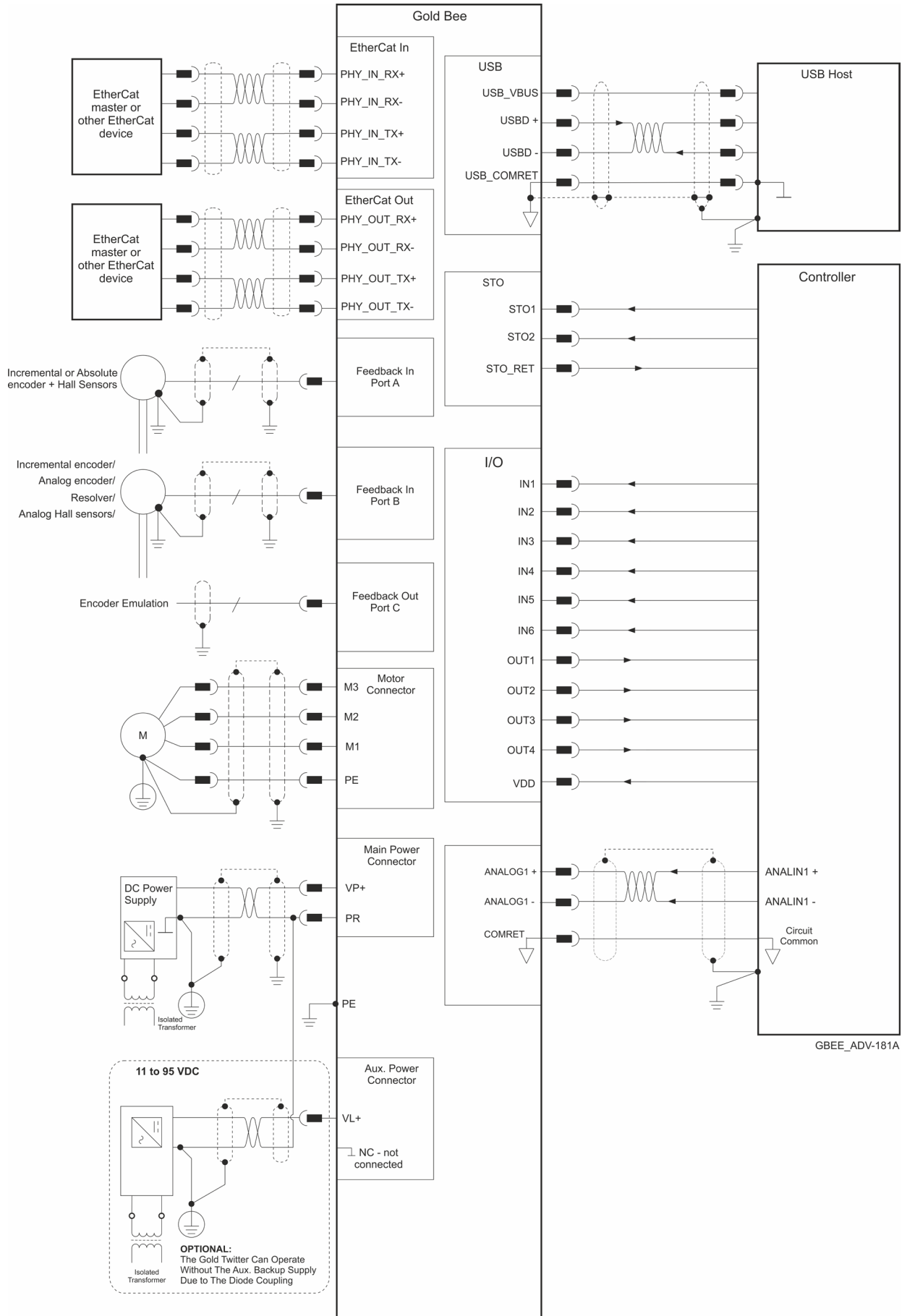
Figure 4: The Gold Bee EtherCAT Connection Diagram
