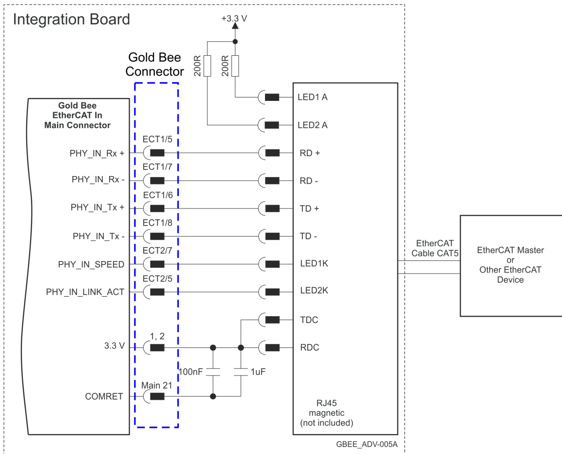
Figure 29: EtherCAT Connection Schematic Diagram
