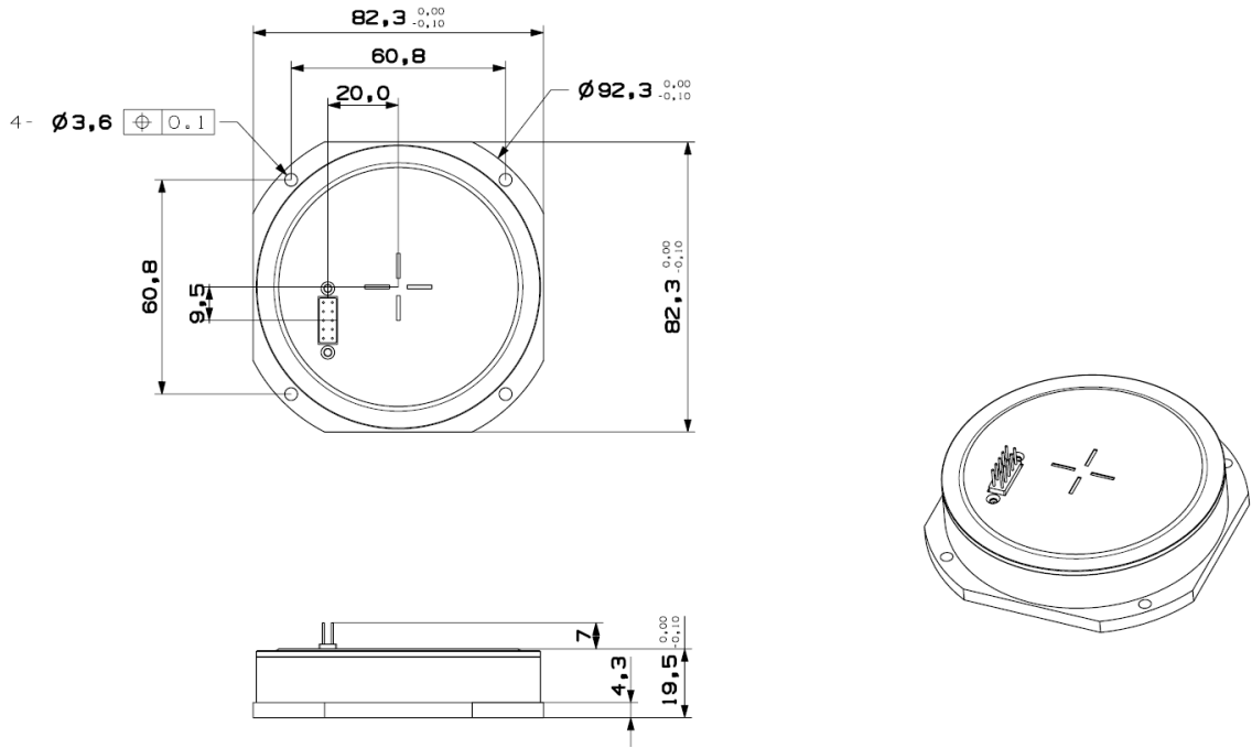
Fig 2 BS-FG91-240-A1EC dimension
