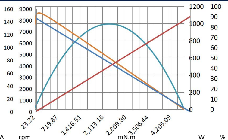
电机特性曲线 (Motor Characteristics Curve)
