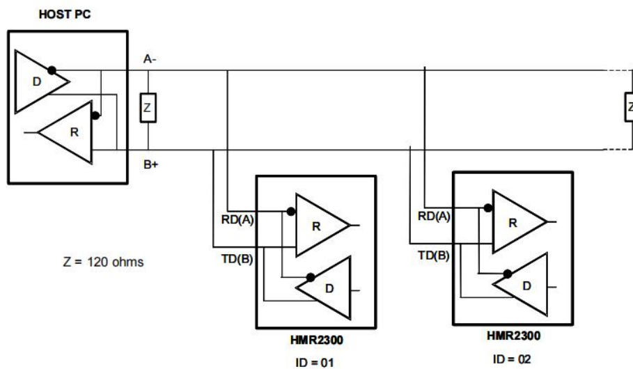
RS-485 BALANCED I/O INTERCONNECTS – Figure 7
