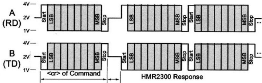
GLOBAL ADDRESS (*99) DELAY – Figure 3 (Timing is Not to Scale)
