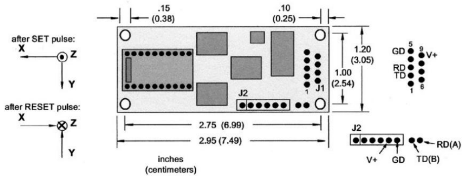
CASE DIMENSIONS – Figure 5
