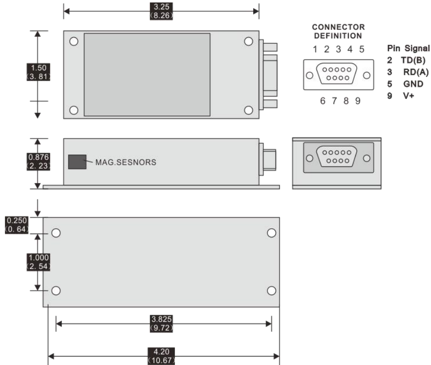
CASE DIMENSIONS – Figure 5
